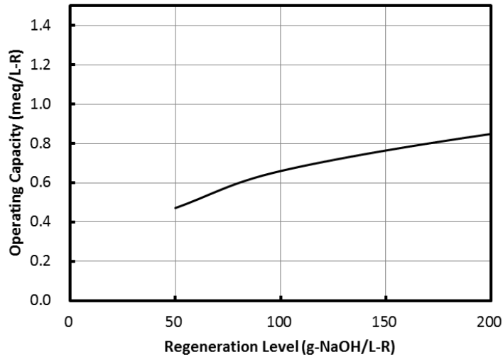
Fig. 3 Operational Capacity Data of UBA10A Regenerant : 4 % NaOH
