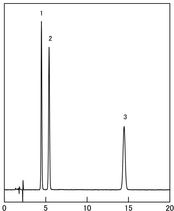
Fig. Chromatogram of β blockers.
