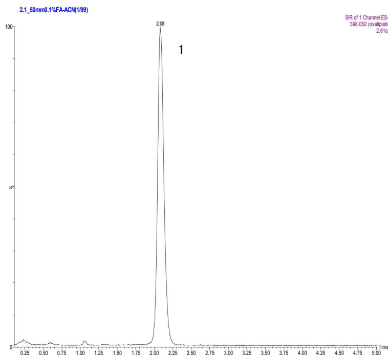
Fig. Chromatogram of Oxaliplatin
