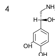
Norepinephrine
