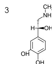
Epinephrine
